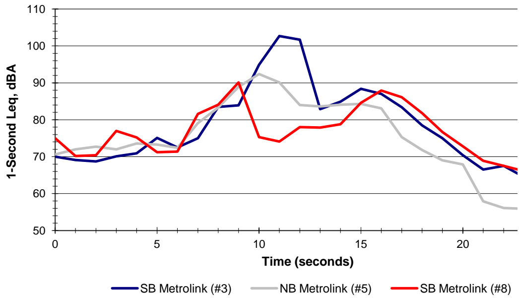
Sound Level vs. Time - Passenger Trains
